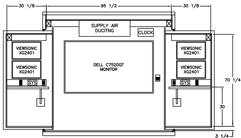
REAR WALL INTERIOR LAYOUT
