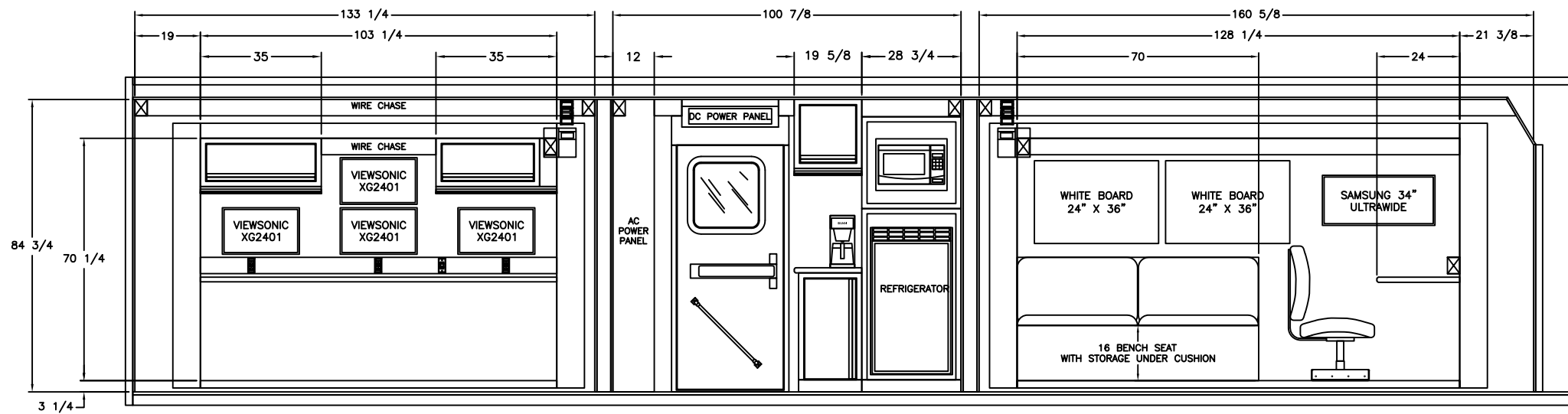
PASSENGERS SIDE INTERIOR LAYOUT
