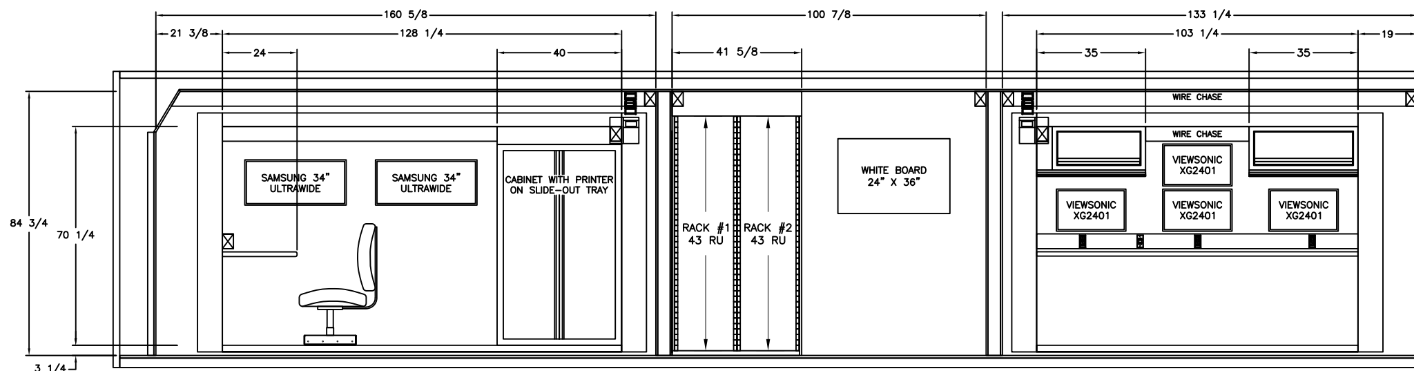
DRIVERS SIDE INTERIOR LAYOUT
