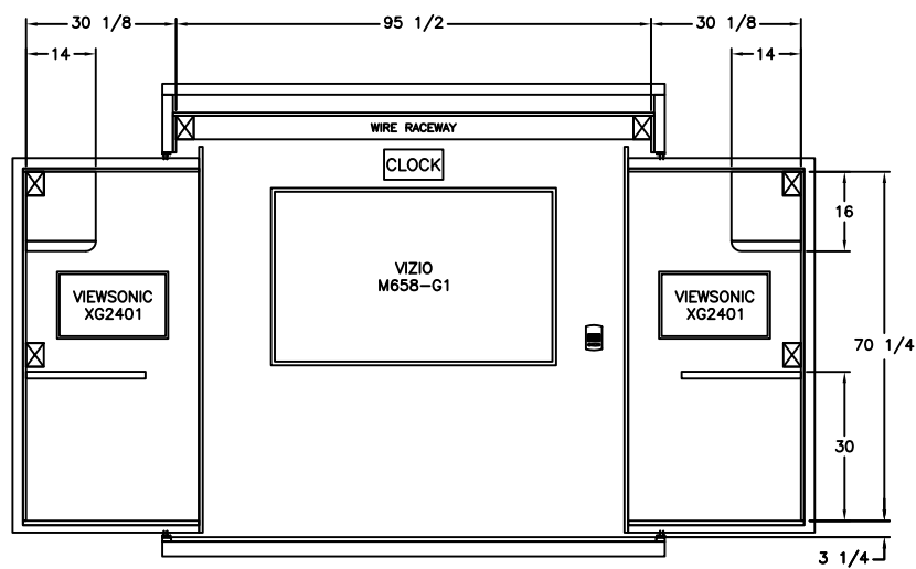
FRONT WALL INTERIOR LAYOUT
