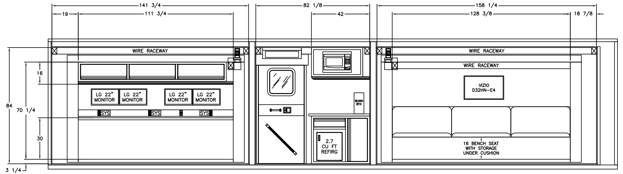
PASSENGER SIDE INTERIOR LAYOUT
