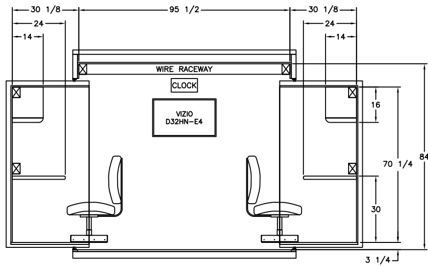
FRONT WALL INTERIOR LAYOUT
