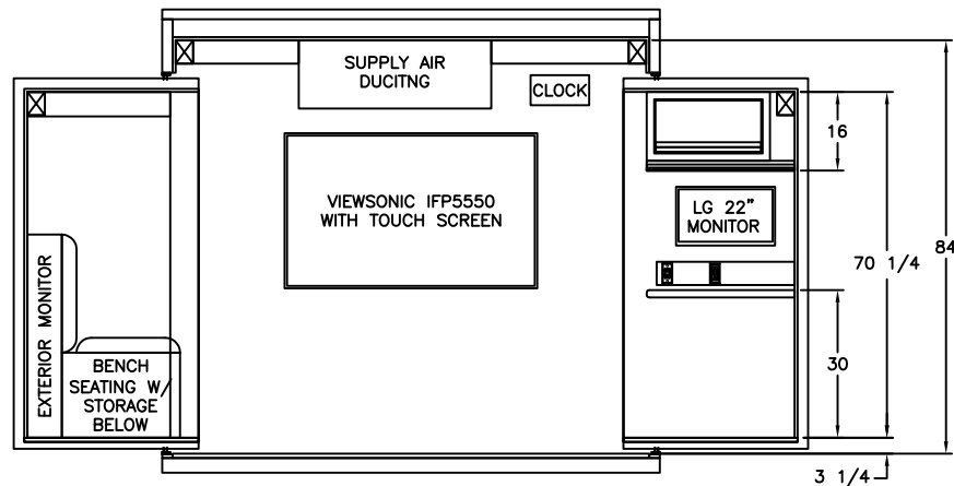
REAR WALL INTERIOR LAYOUT
