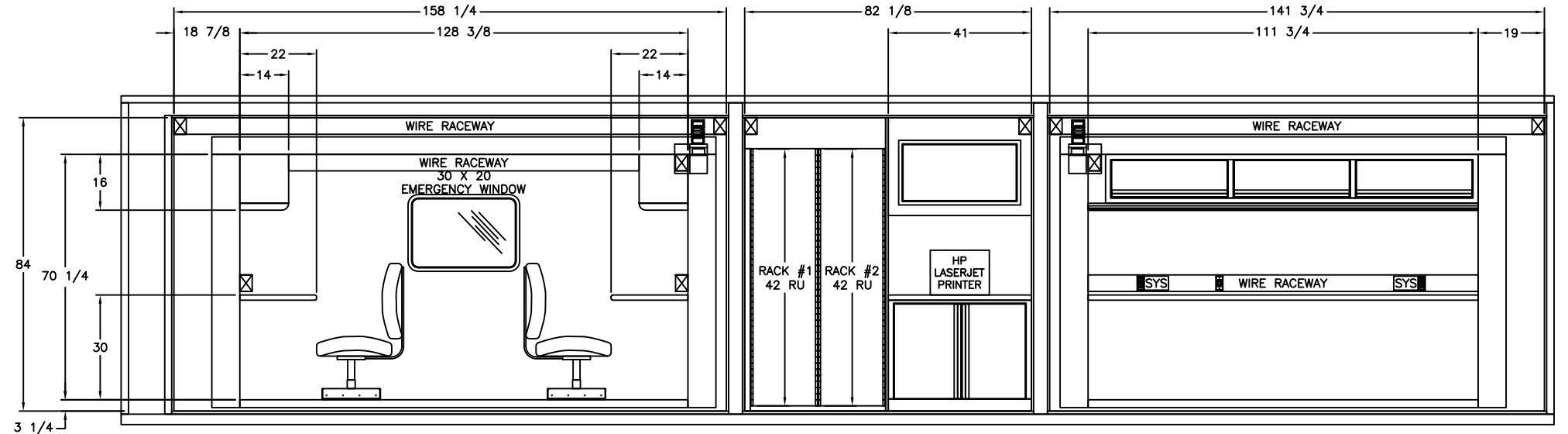
DRIVER SIDE INTERIOR LAYOUT
